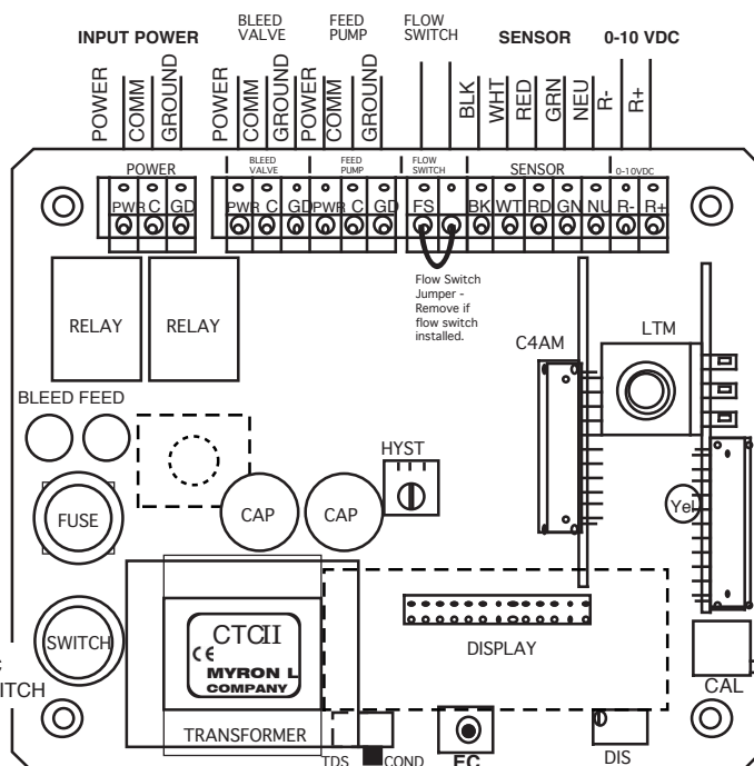
ELECTRICAL CONNECT DIAGRAM Figure II.E.1
