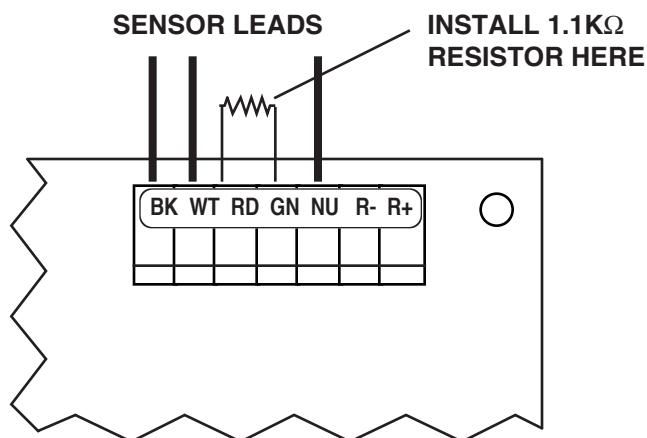
Main CB Assembly
