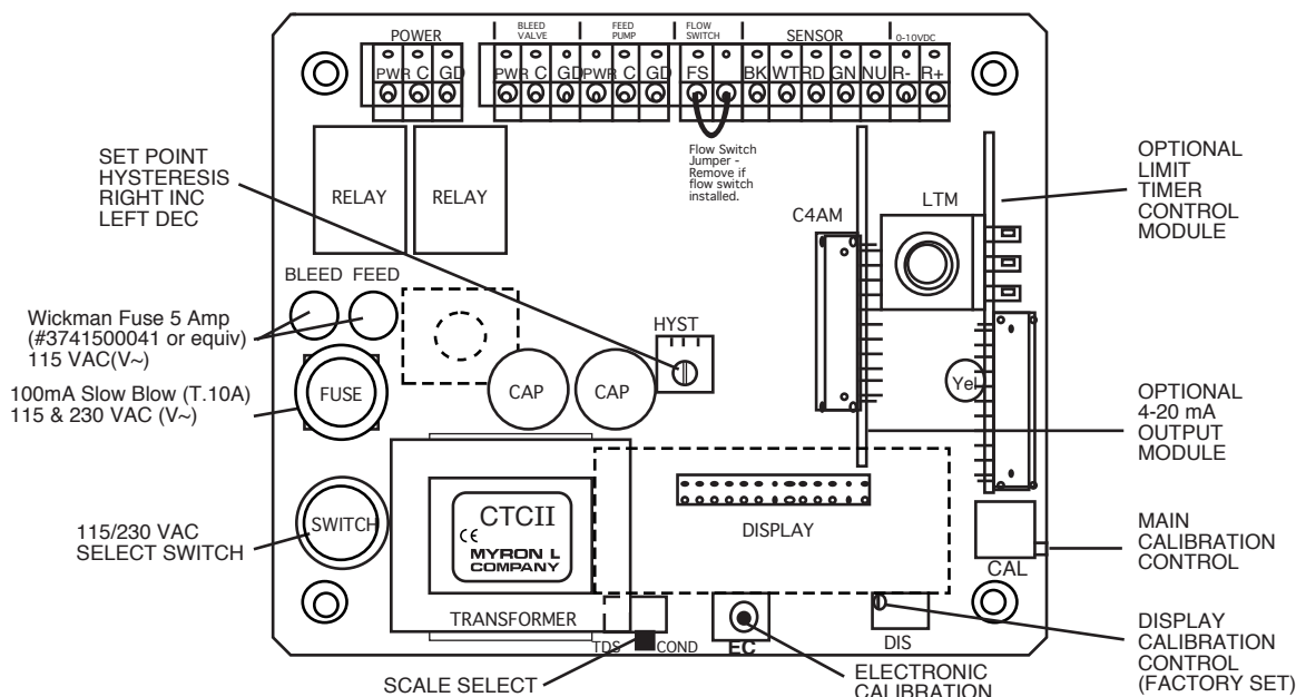
CTCII MAIN CIRCUIT BOARD
