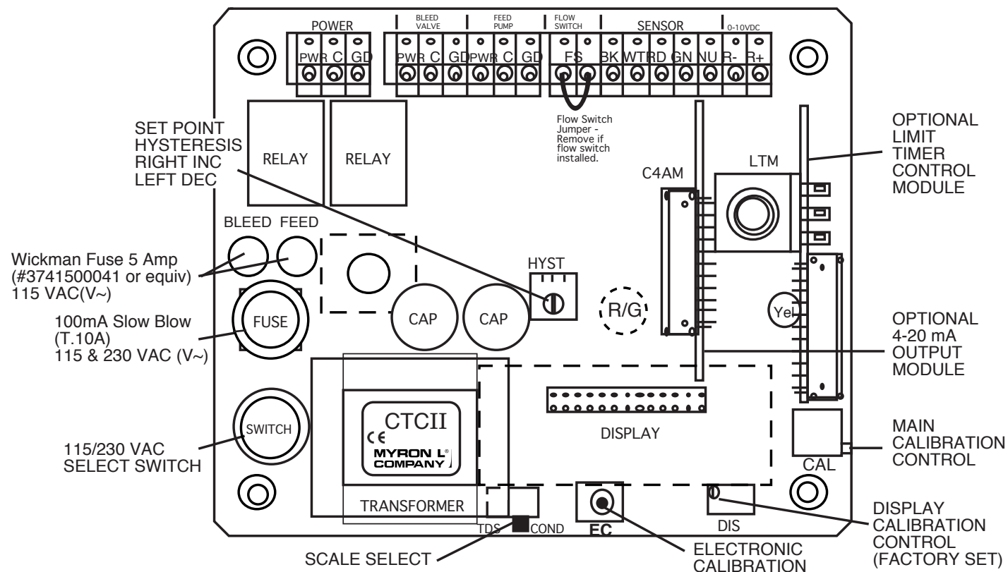
CTCII MAIN CIRCUIT BOARD
